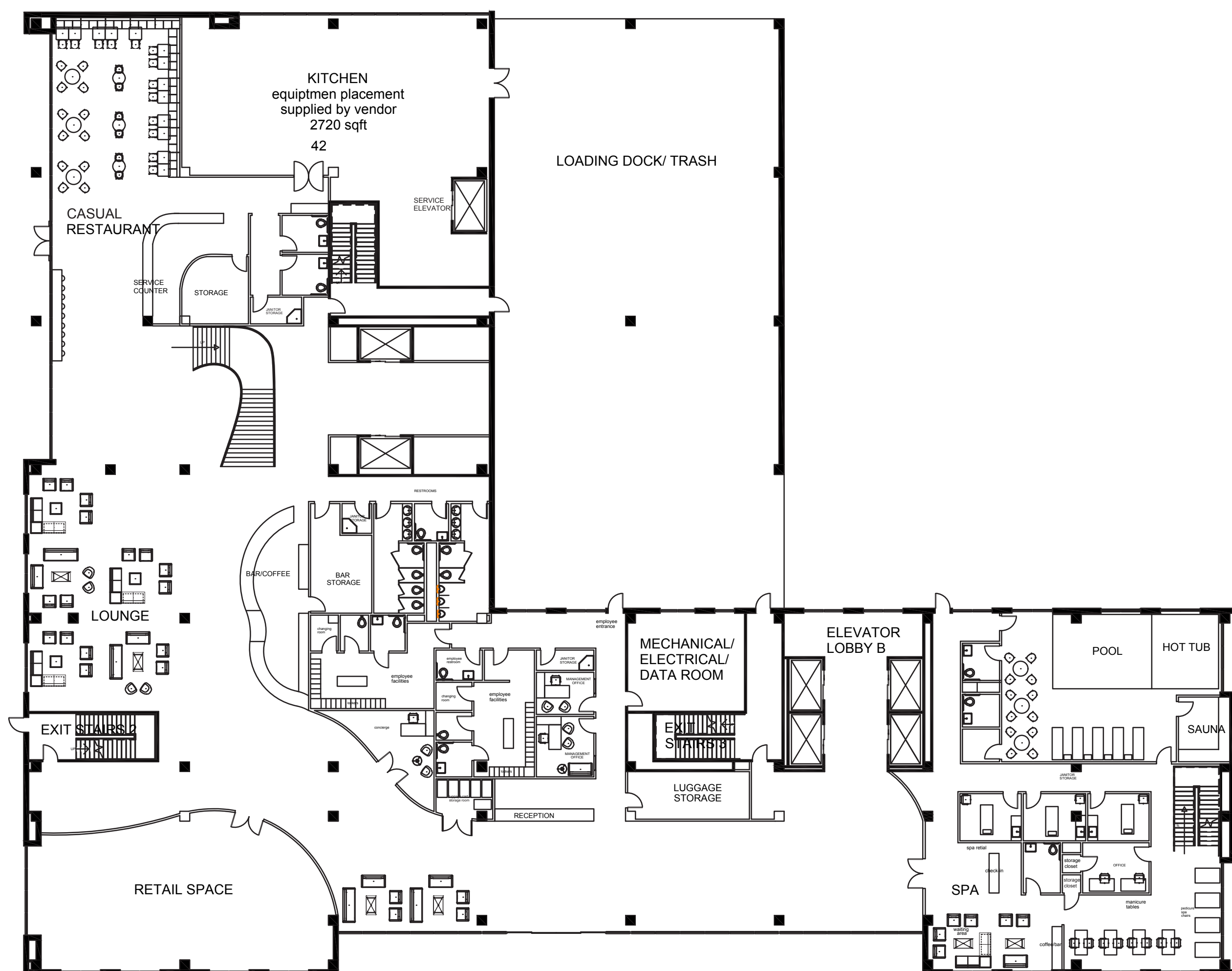
1ST FLOOR FURNITURE PLAN
