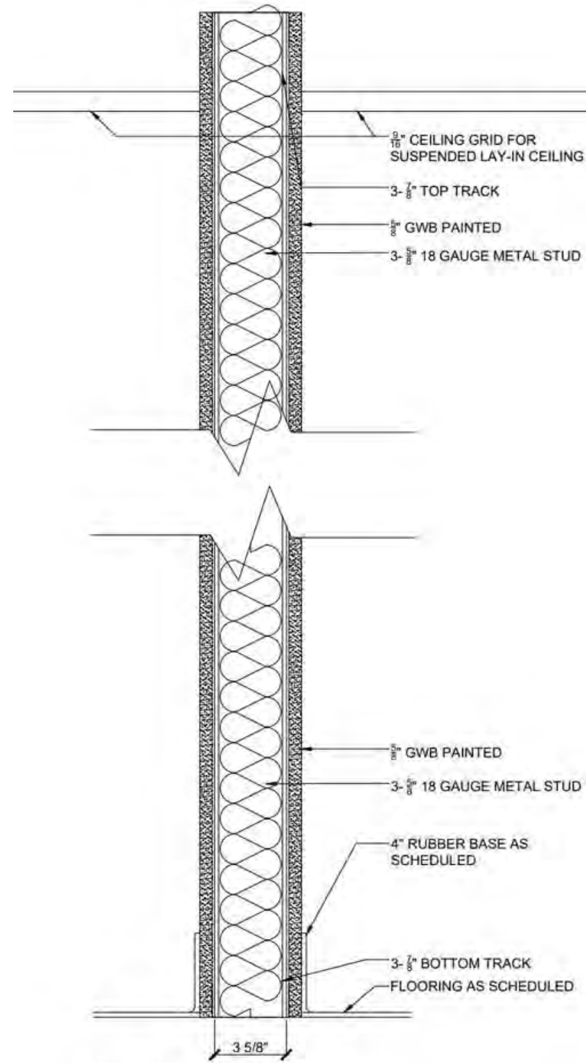
INSULATED WALL SECTION
