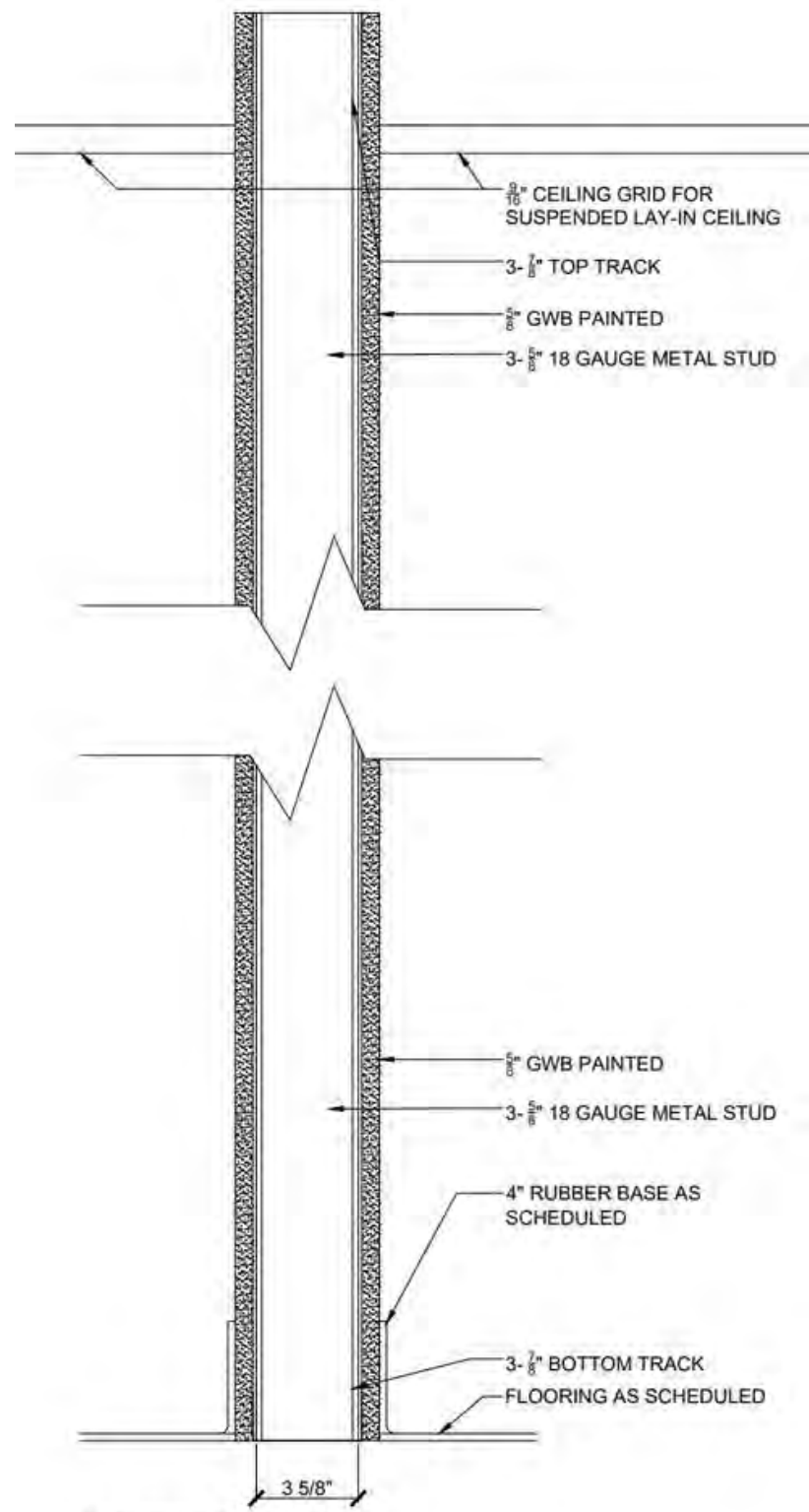
STANDARD WALL SECTION
