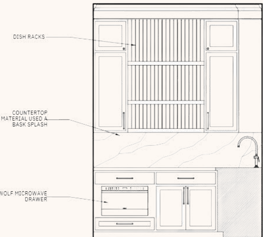
K. Scullery Microwave Elevation
