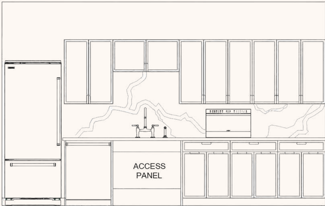
Break Room Elevation
