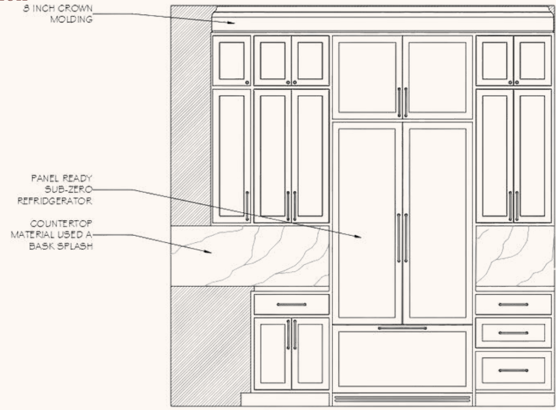
Fridge Elevation
