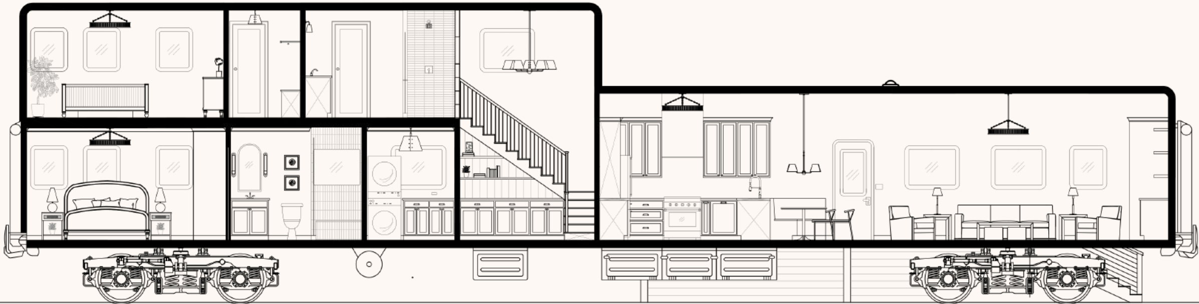
Interior Section
