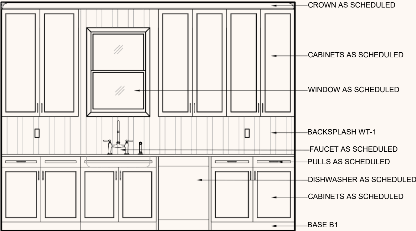
Kitchen Sink Elevation
