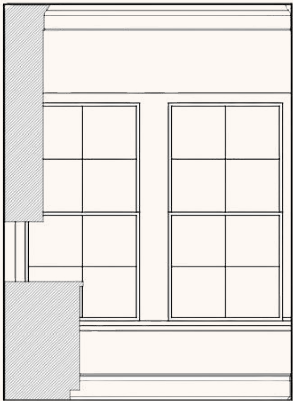
I.Scullery Window Elevation
