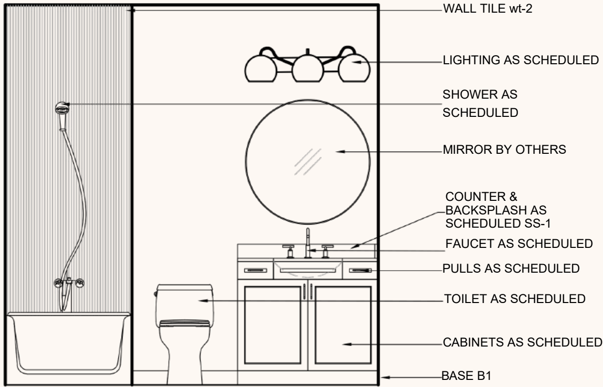
Bathroom Elevation
