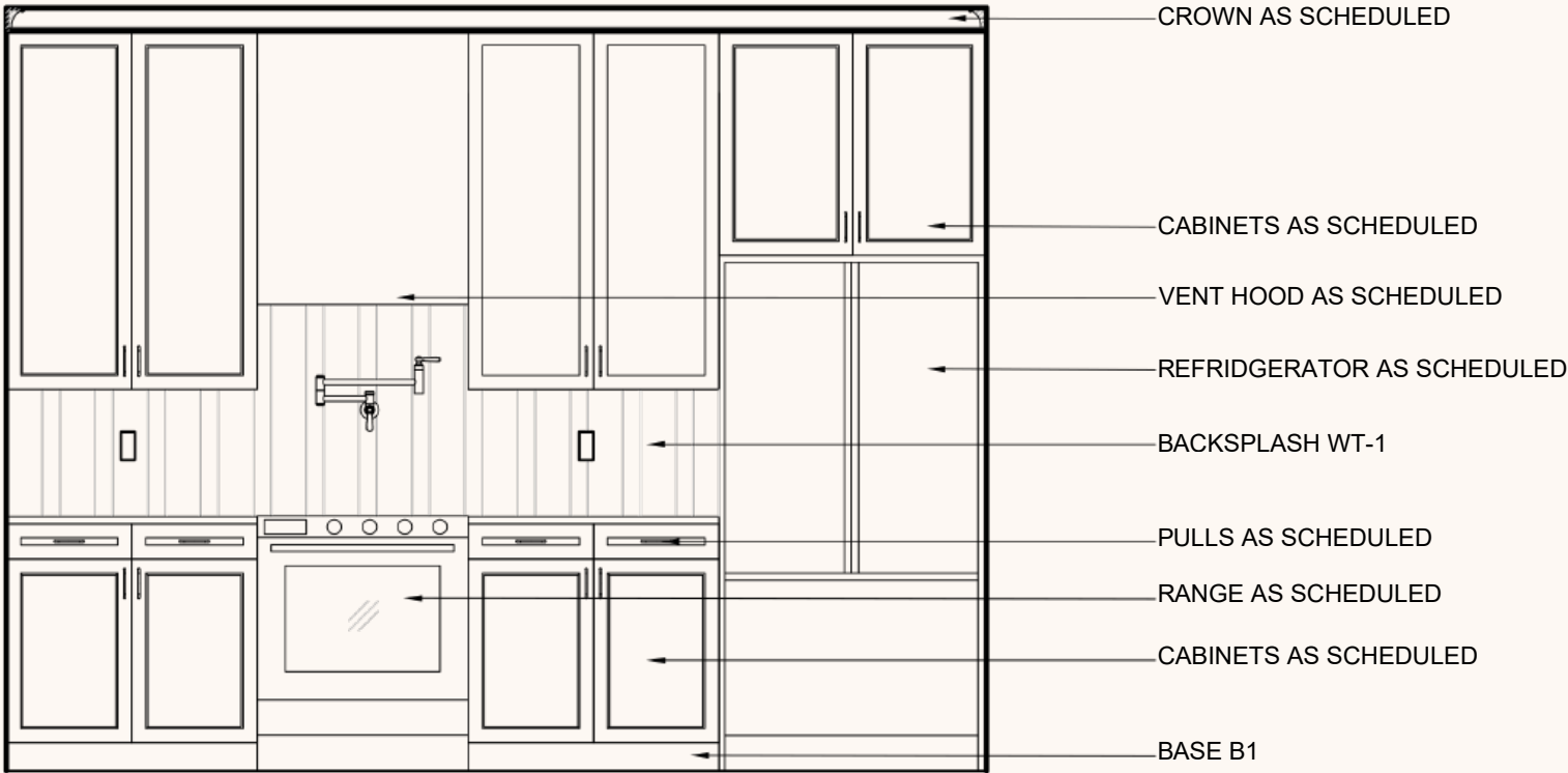
Kitchen Range Elevation
