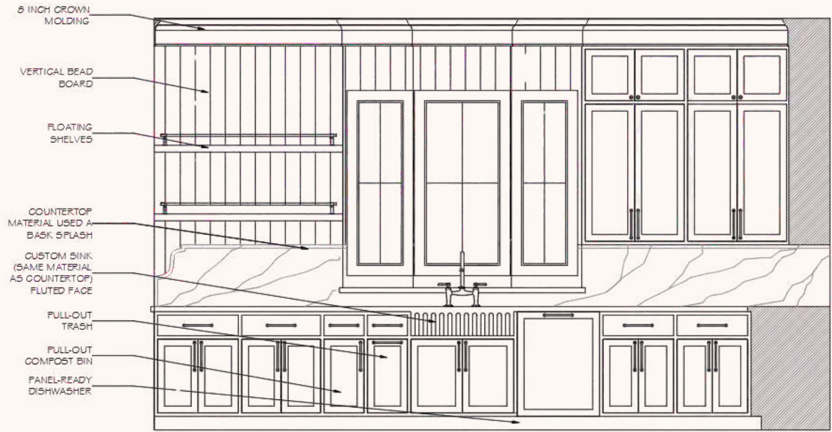
Sink Elevation
