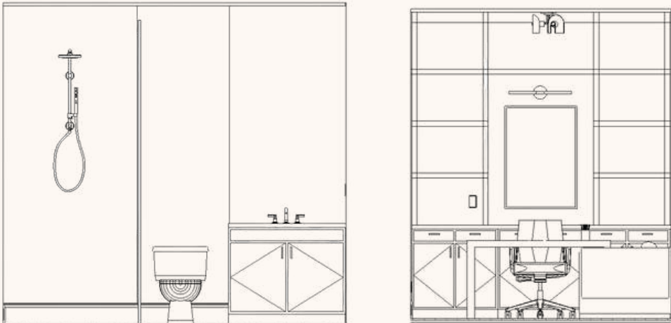
Guest Bathroom and Office Elevations
