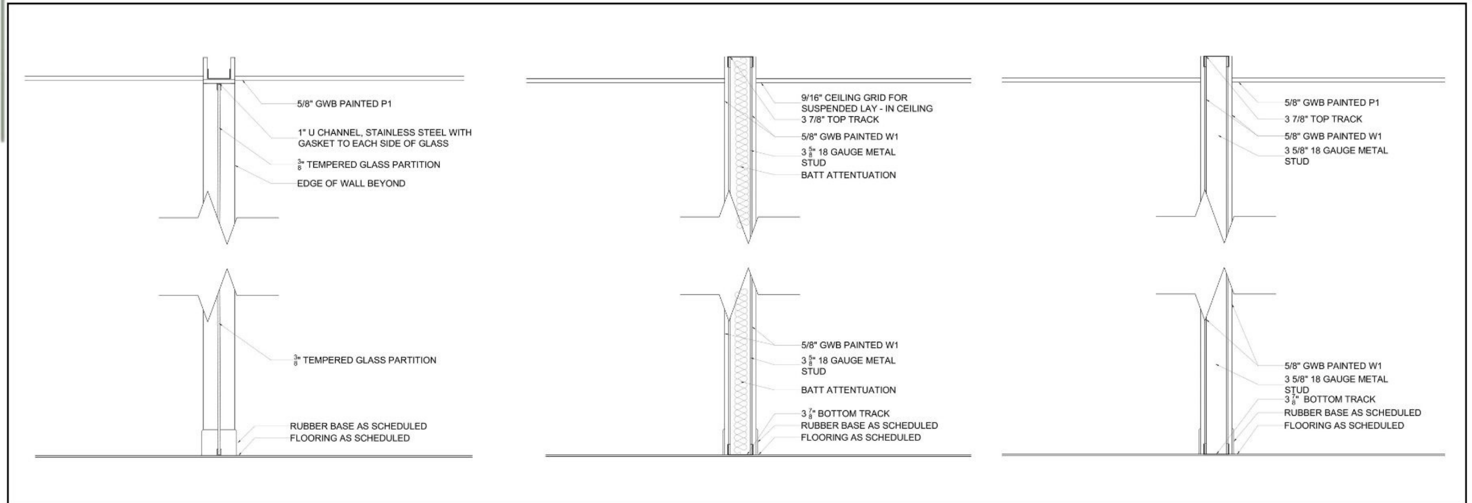
Glass wall section
