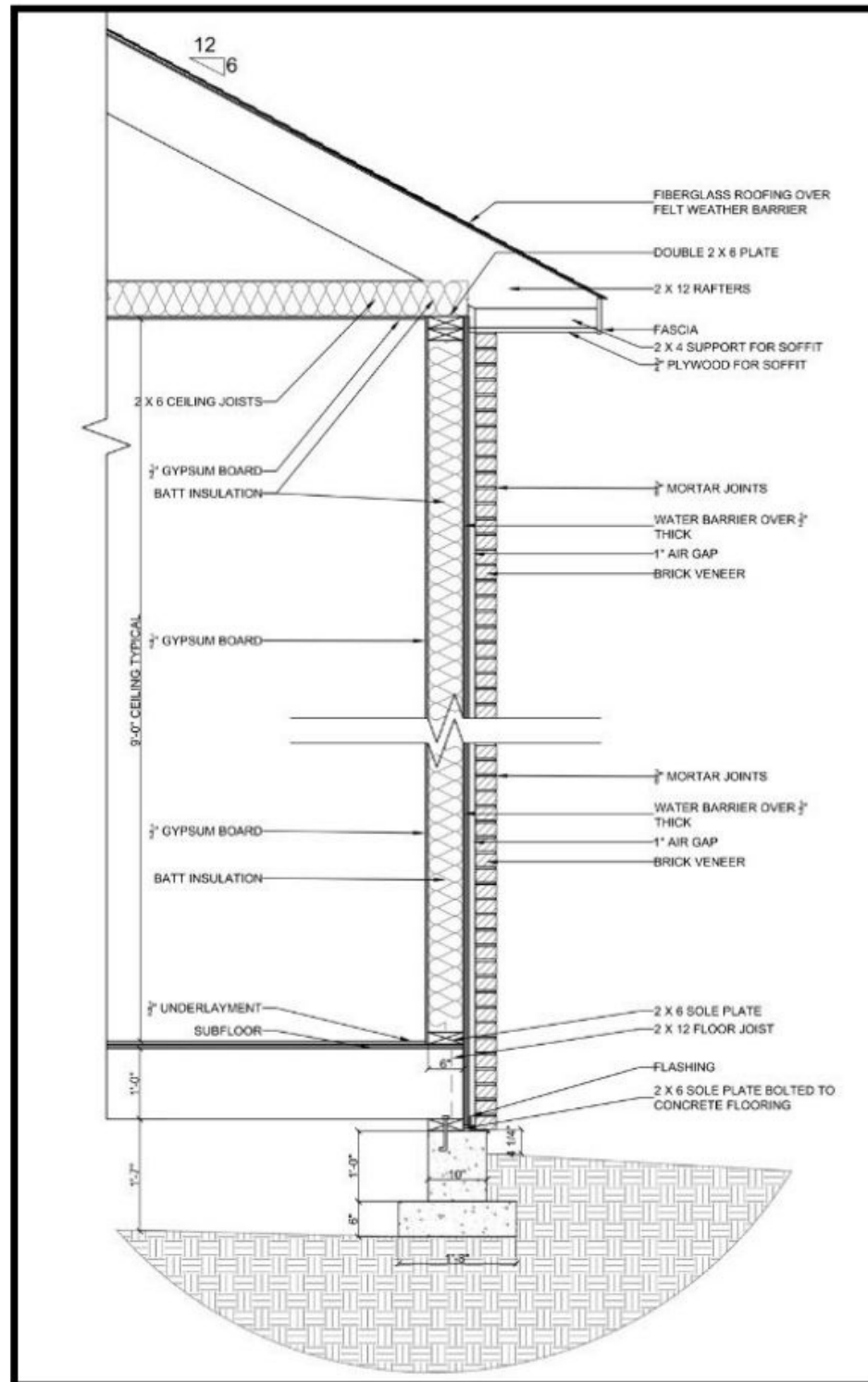
Exterior Detail
