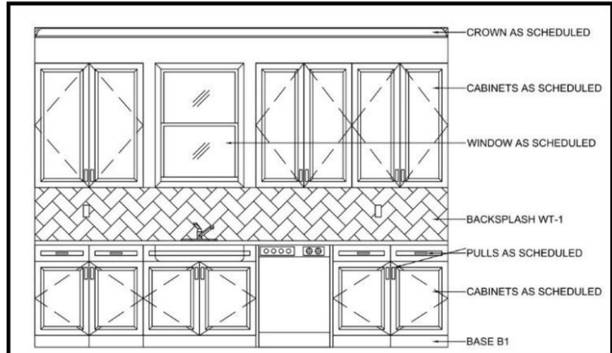
Kitchen Elevation
