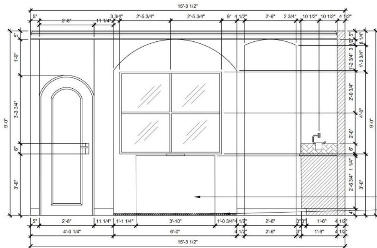
Elevation H
