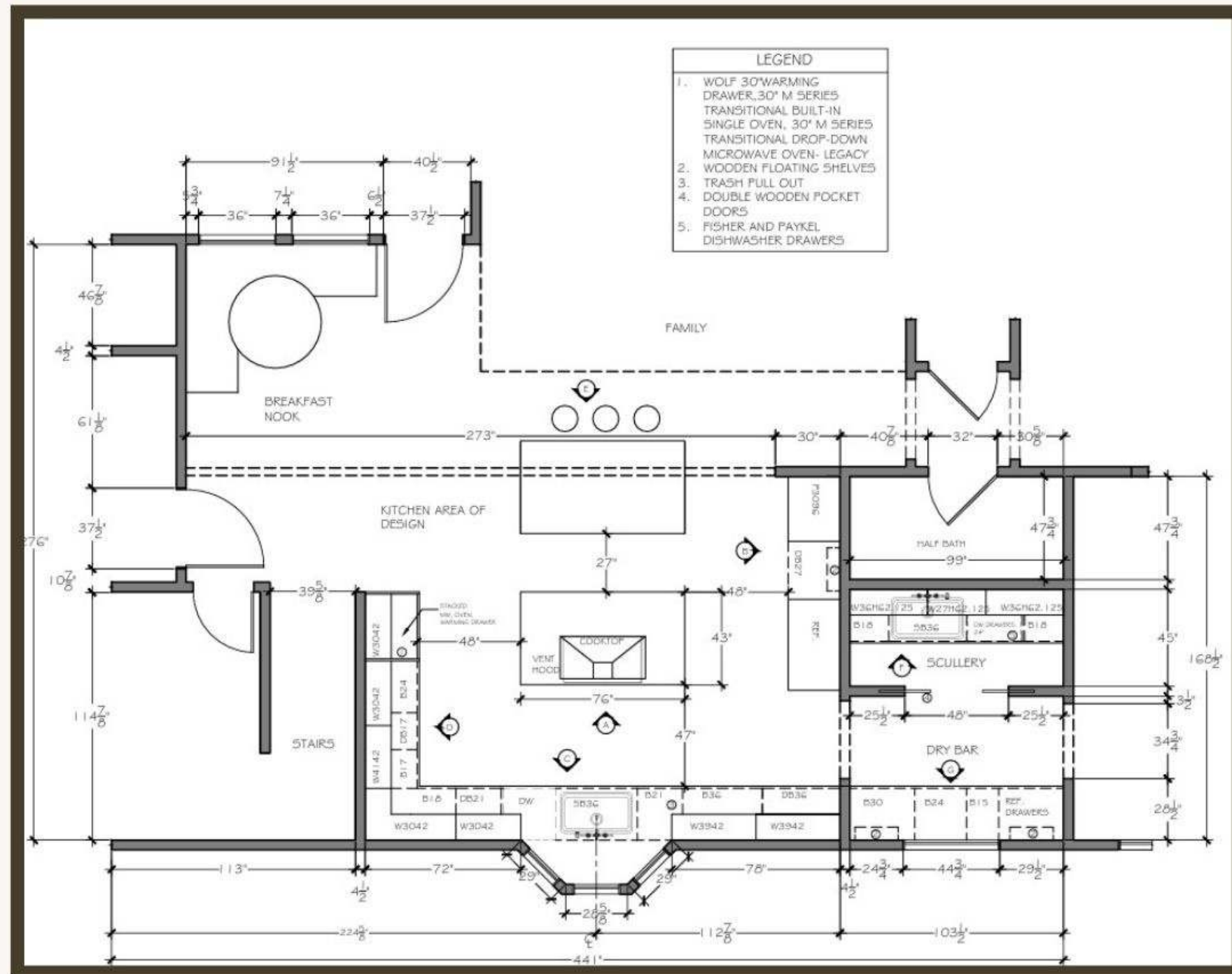
FLOORPLAN
