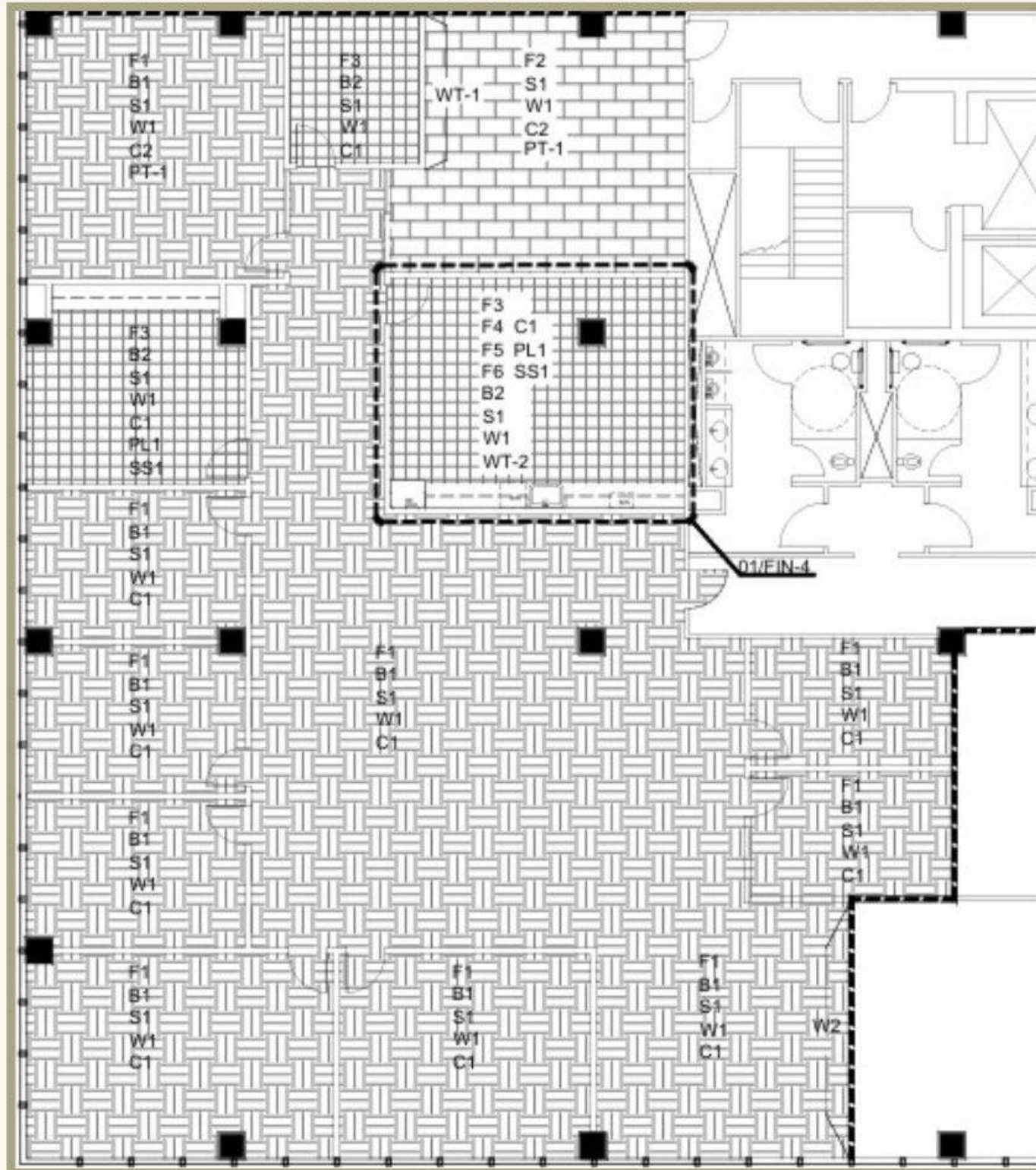
FINISH PLAN
