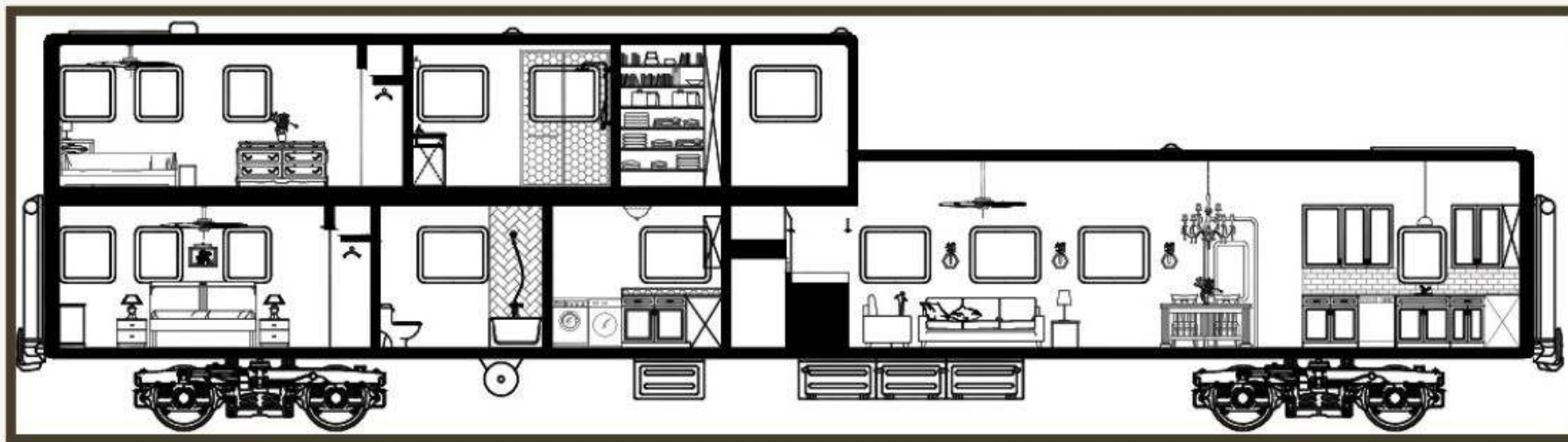
SECTION
