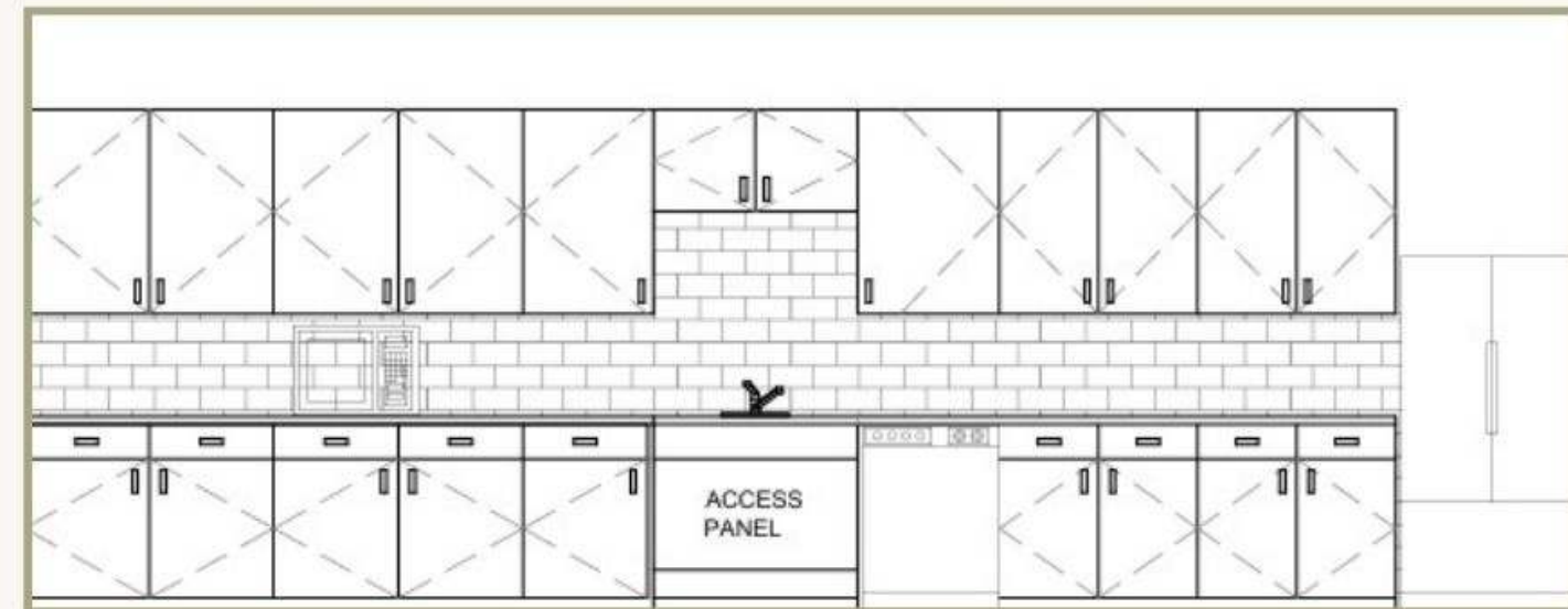
BREAK ROOM ELEVATION
