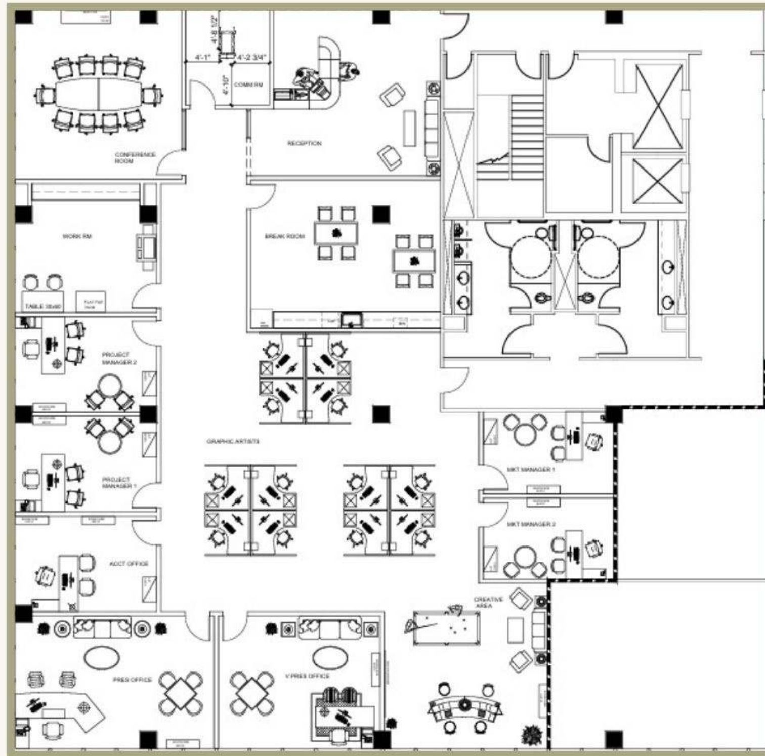
FURNITURE PLAN
