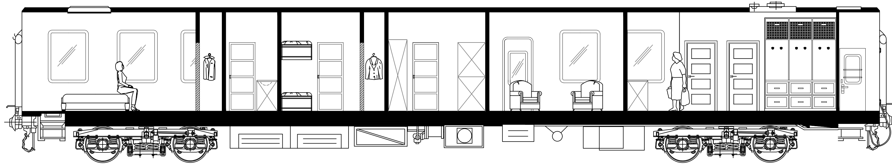
01 FRONT SECTION SCALE: 3/16" = 1'-0"
