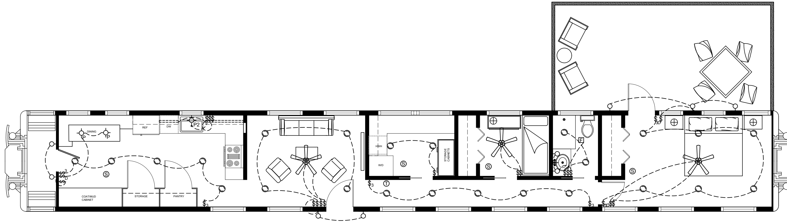
01 LIGHTING PLAN SCALE: 3/16" = 1'-0"
