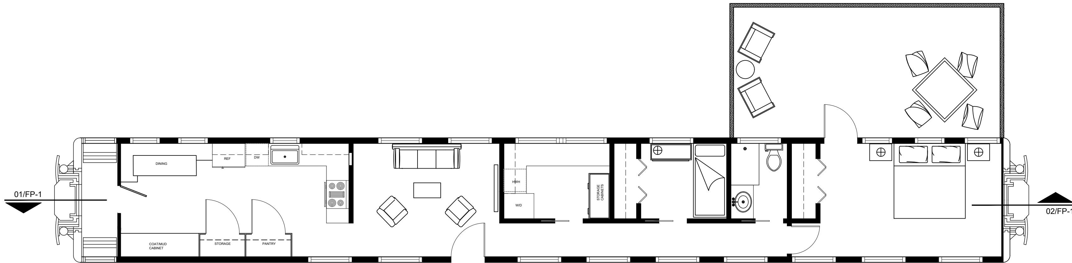
01 FLOOR PLAN SCALE: 3/16" = 1'-0"
