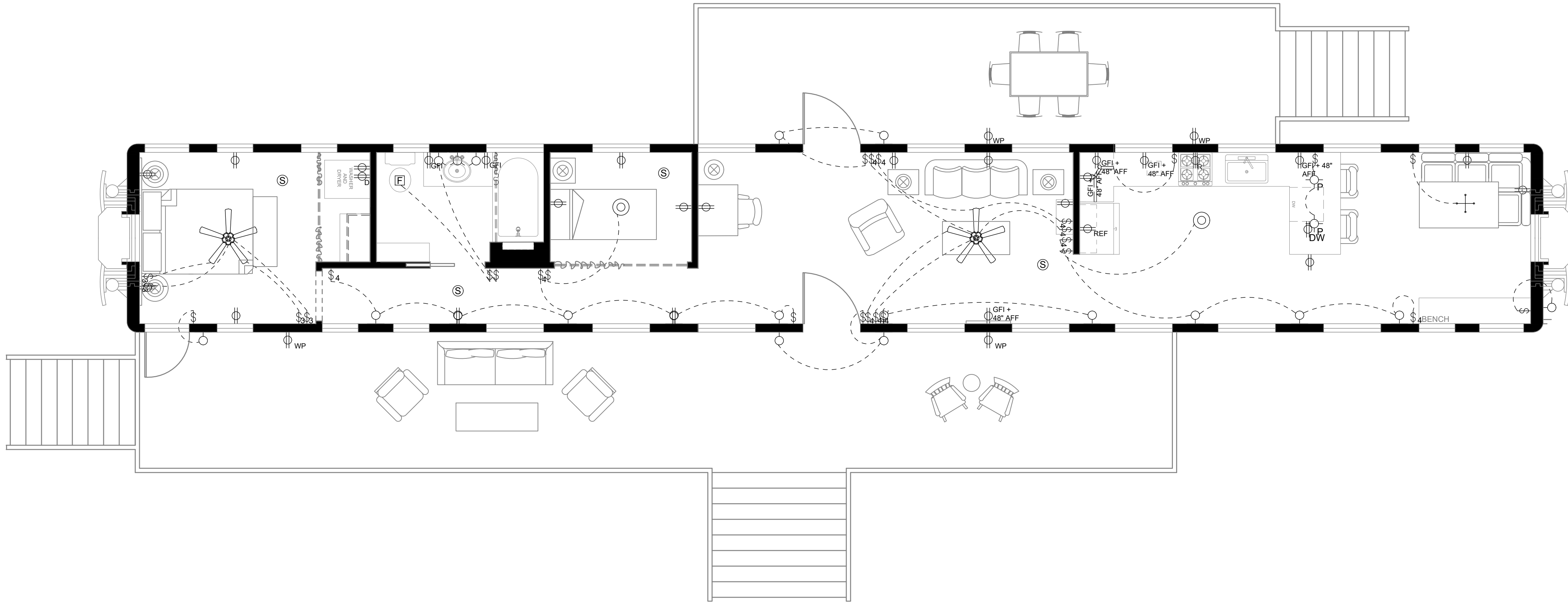
01 LIGHTING PLAN SCALE: 1/4" = 1'-0"
