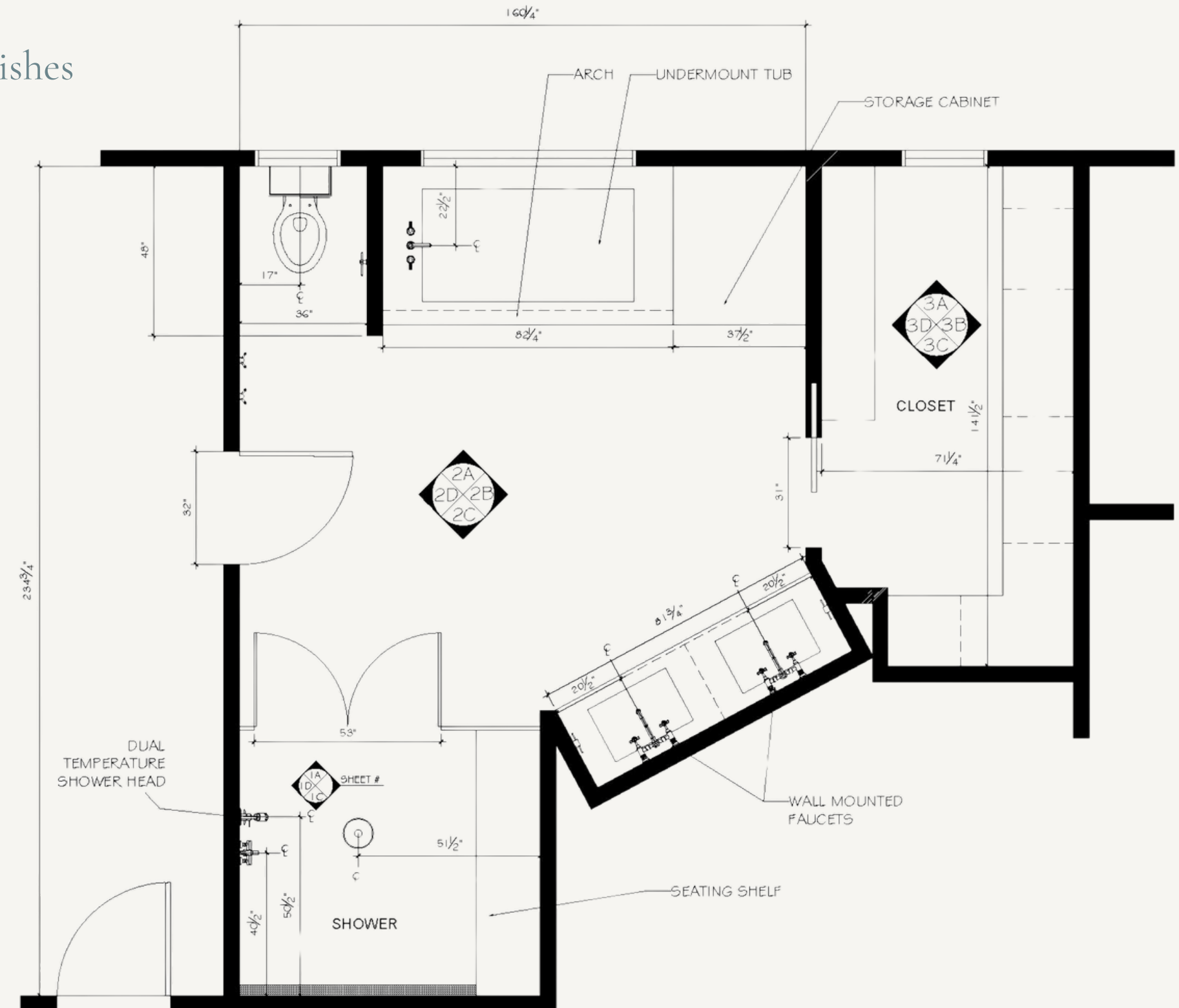
FLOOR PLAN
