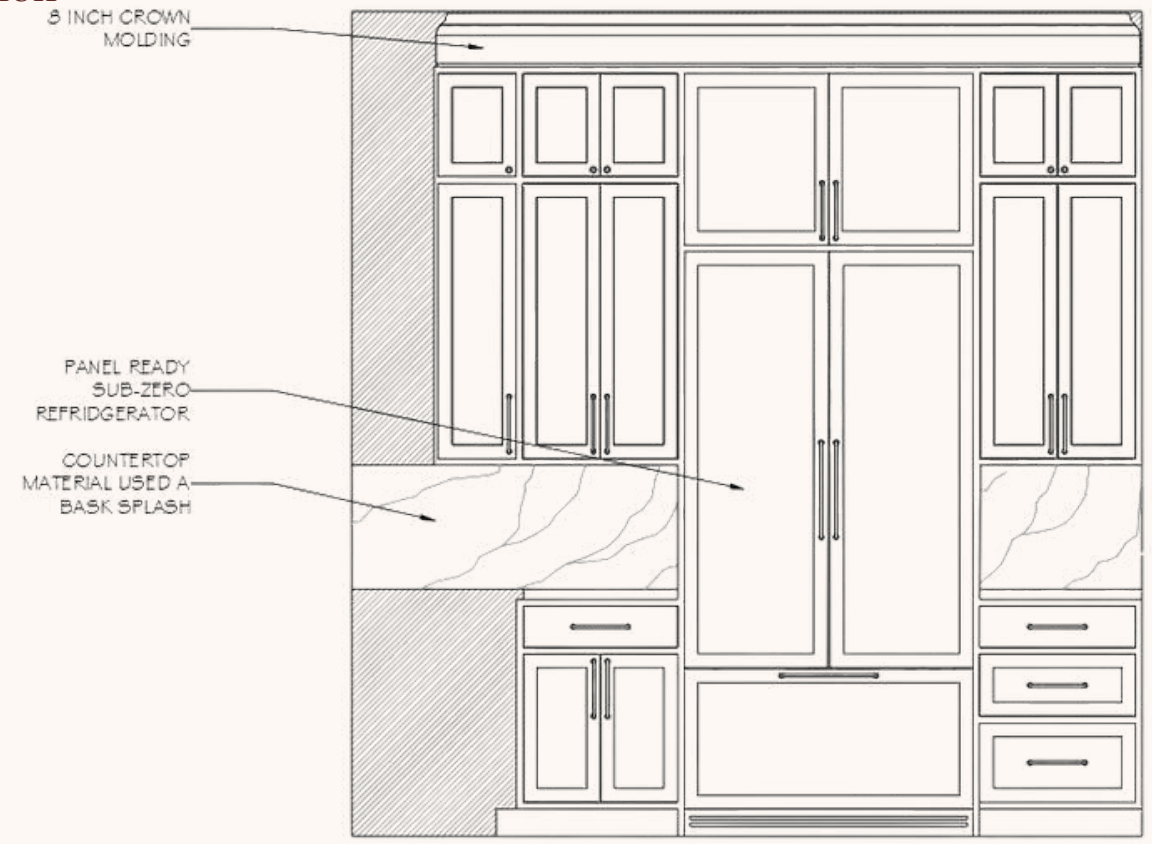
Fridge Elevation
