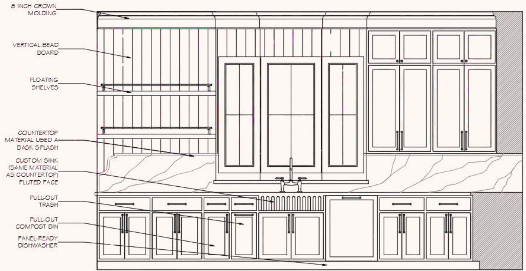
Sink Elevation
