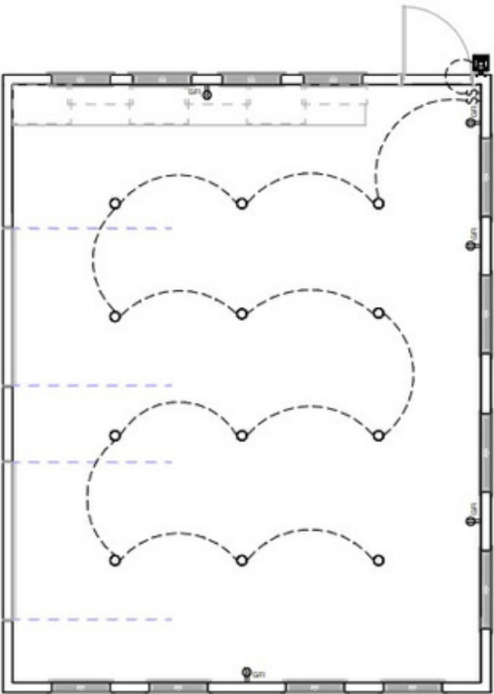
ELECTRICAL/LIGHTING PLAN
