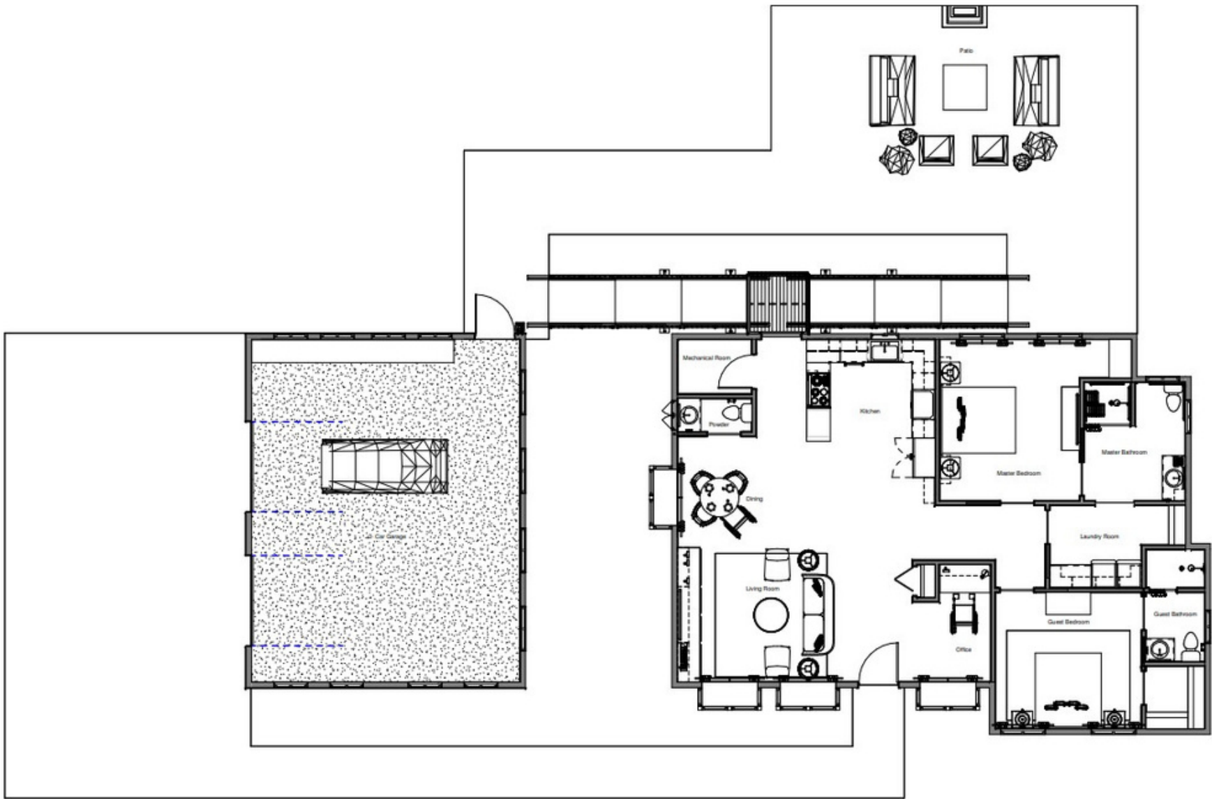
FURNITURE PLAN
