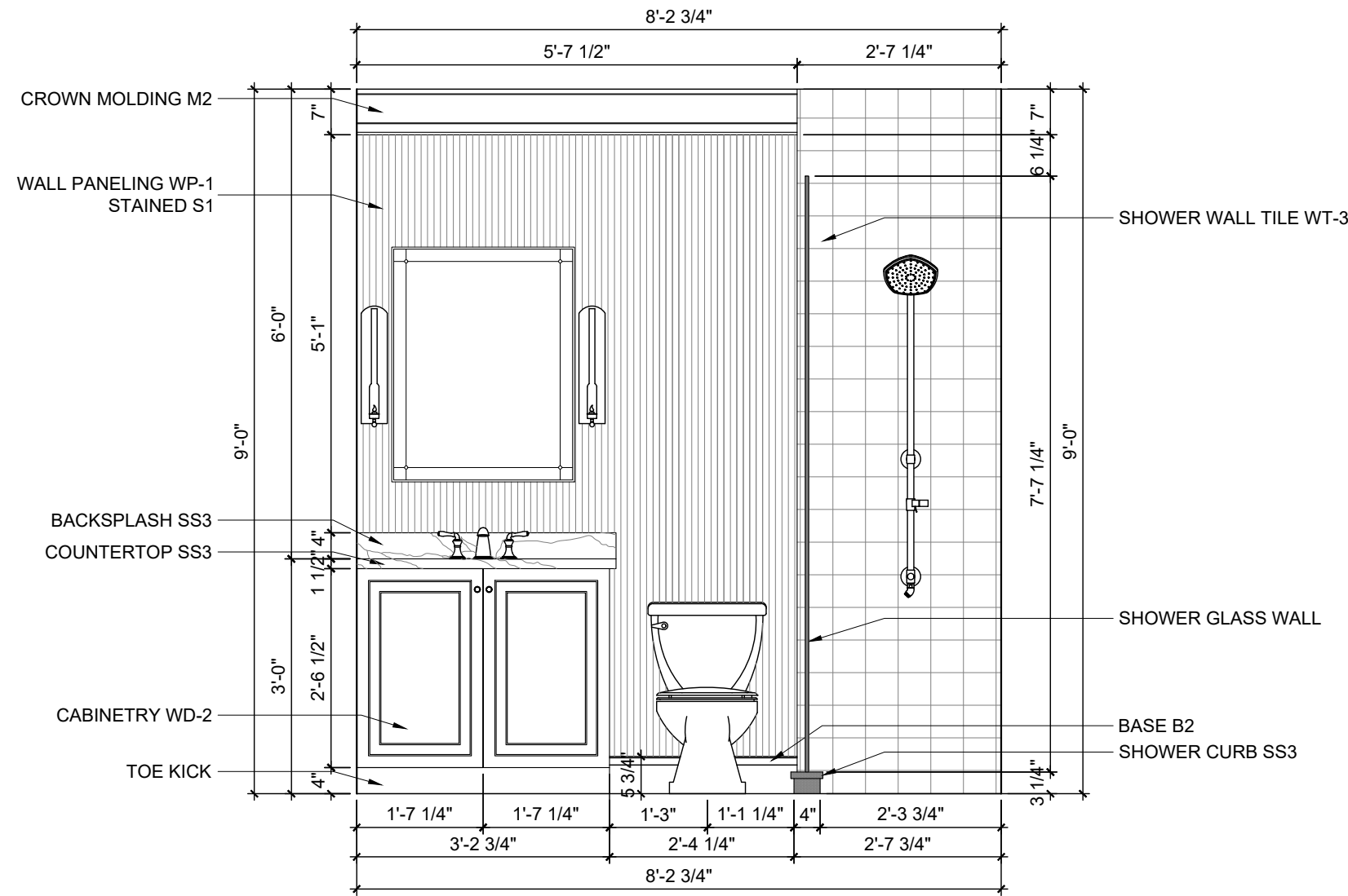
K MASTER BATH SINK ELEV. SCALE: \frac{1}{2}" = 1' - 0"
