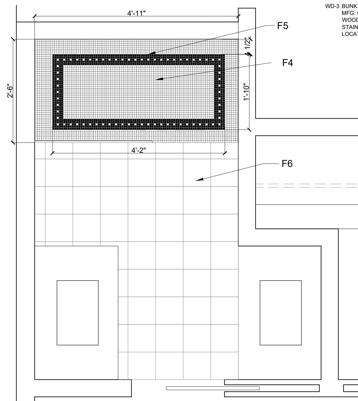
01 MASTER BATHROOM FLOOR DETAIL SCALE: 3/4" = 1'-0"
