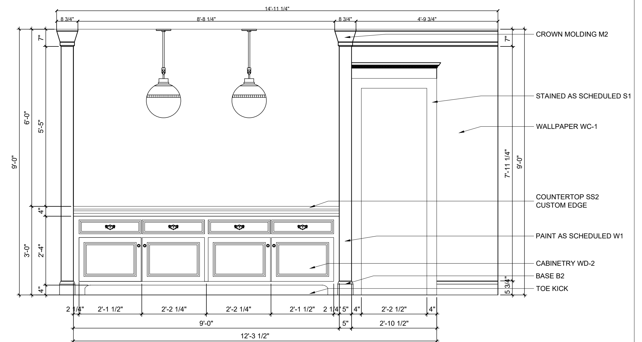
D ISLAND FRONT ELEVATION SCALE: \frac{1}{2}" = 1'-0"
