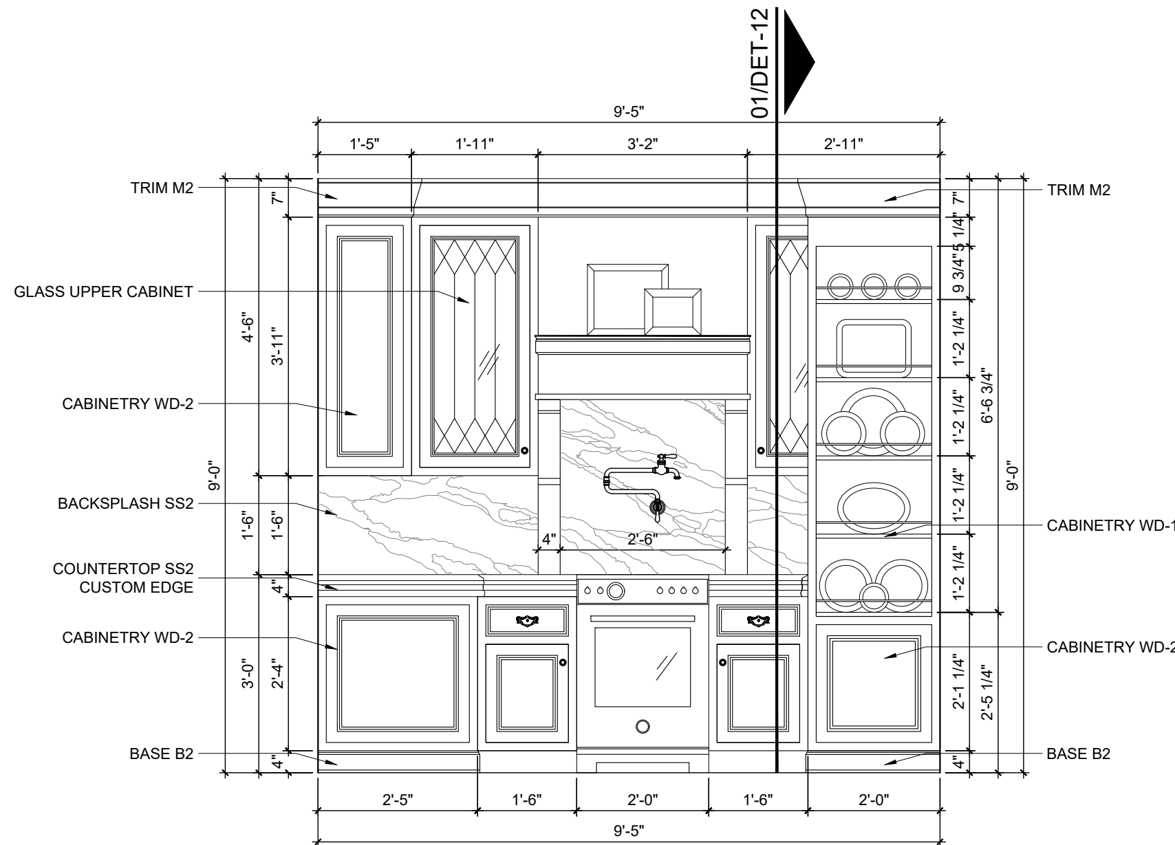
B KITCHEN OVEN ELEVATION SCALE: \frac{1}{2}" = 1'-0"
