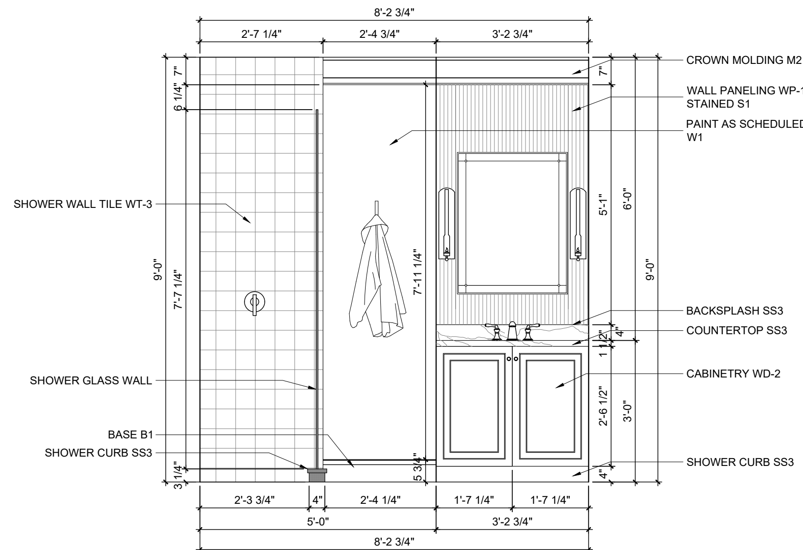
I MASTER SINK ELEV. SCALE: \frac{1}{2}" = 1' - 0"
