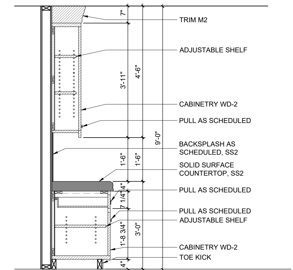
01 CABINET SECTION SCALE: \frac{3}{4}" = 1'-0"
