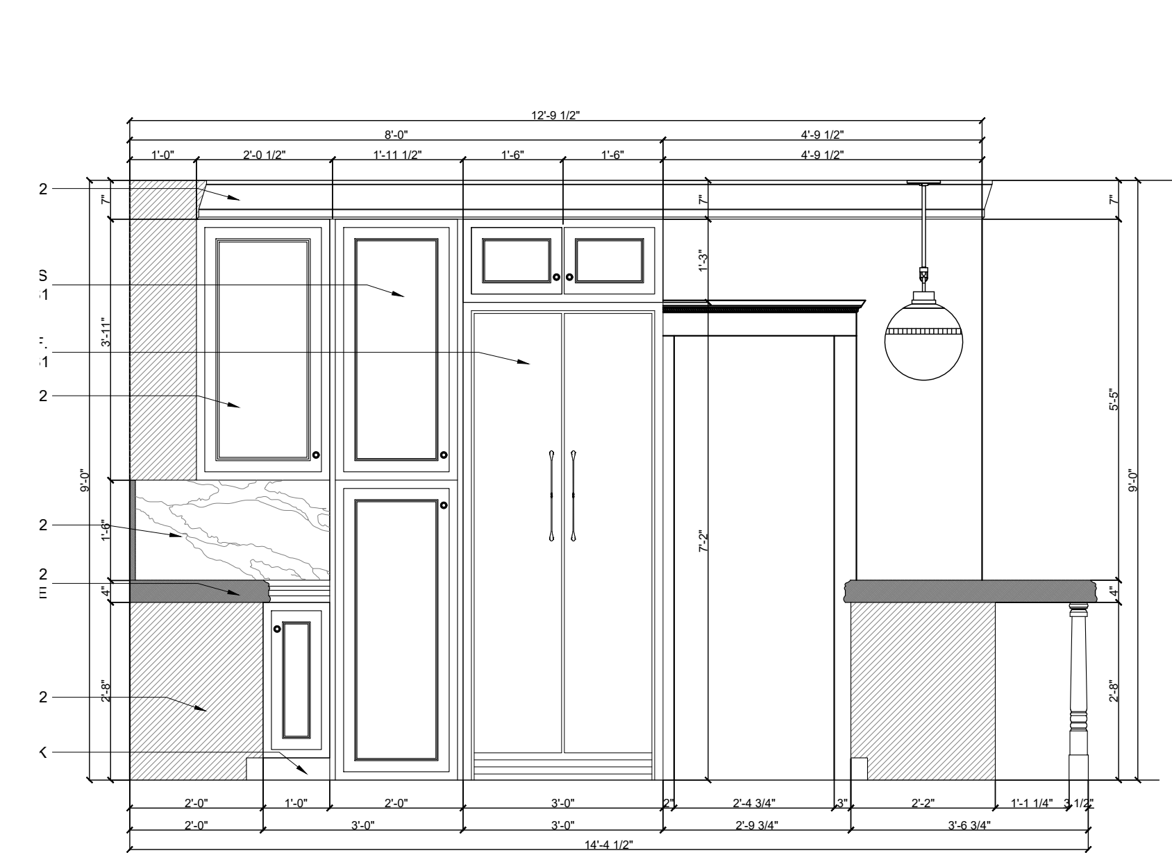
C KITCHEN REF. ELEVATION SCALE: \frac{1}{2}" = 1'-0"
