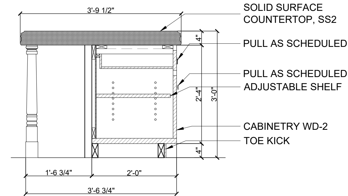
02 KITCHEN ISLAND SECTION SCALE: \frac{3}{4}" = 1'-0"
