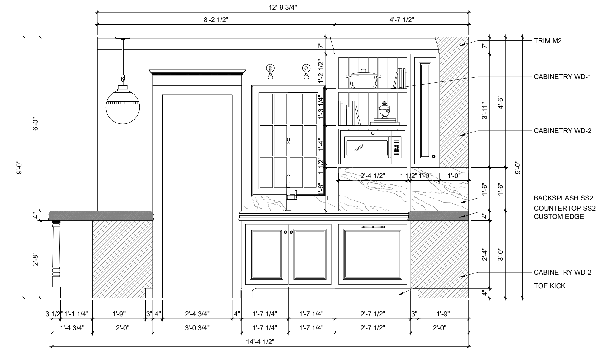
A KITCHEN SINK ELEVATION SCALE: \frac{1}{2}" = 1'-0"
