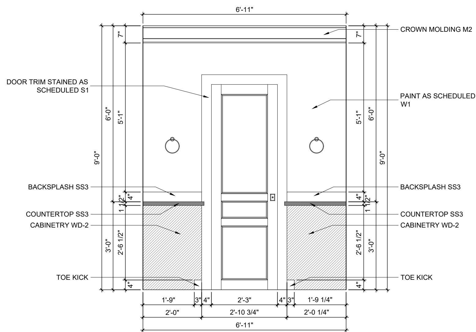
J MASTER BATH ENTRY ELEV. SCALE: \frac{1}{2}" = 1' - 0"
