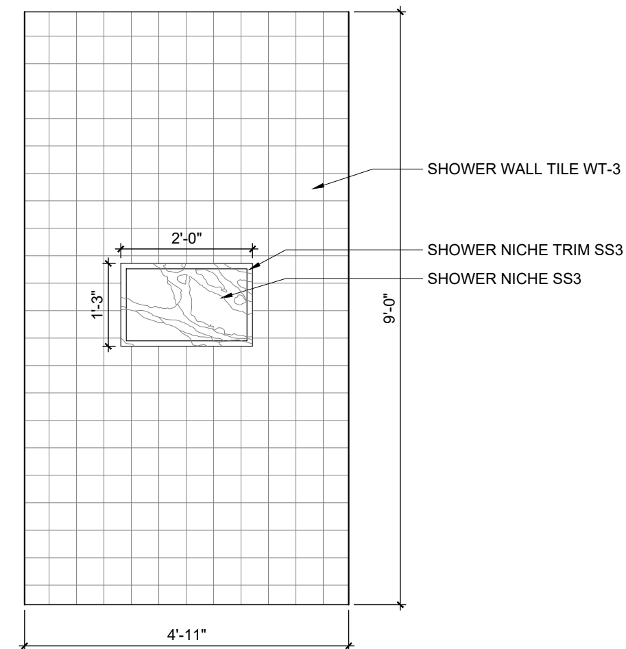
H MASTER SHOWER ELEV. SCALE: \frac{1}{2}" = 1' - 0"
