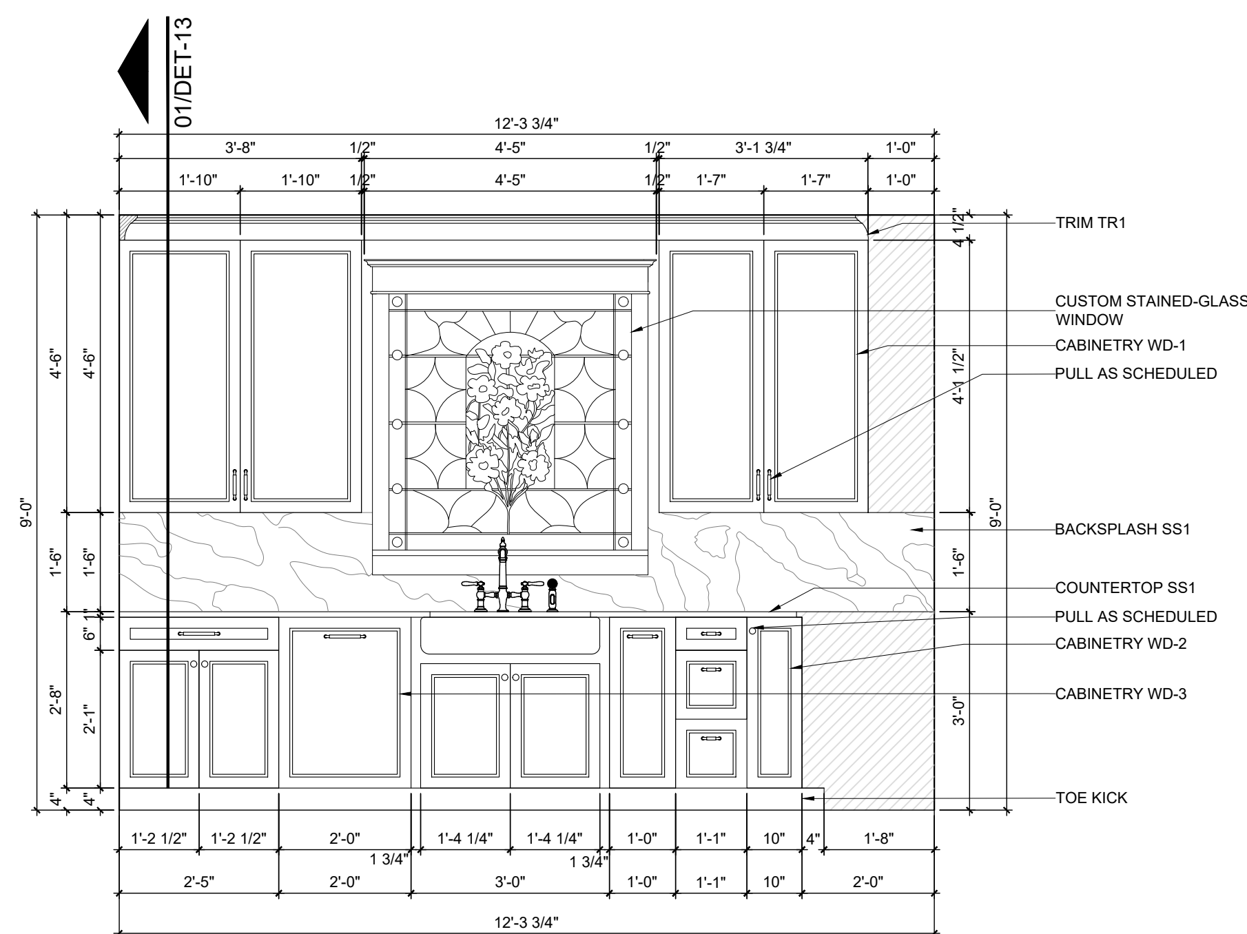
B KITCHEN SINK ELEVATION SCALE: \frac{1}{8}" = 1' - 0"
