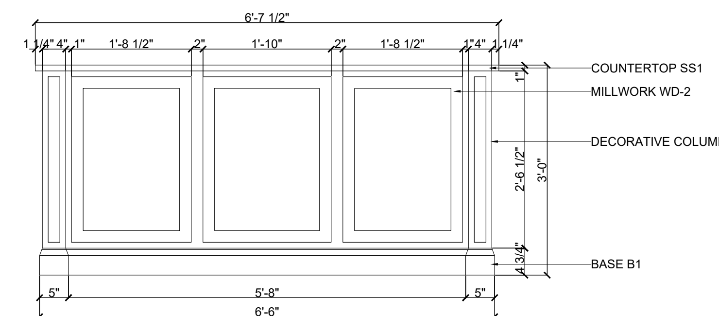
D BACK ISLAND ELEV. SCALE: \frac{1}{8}" = 1' - 0"
