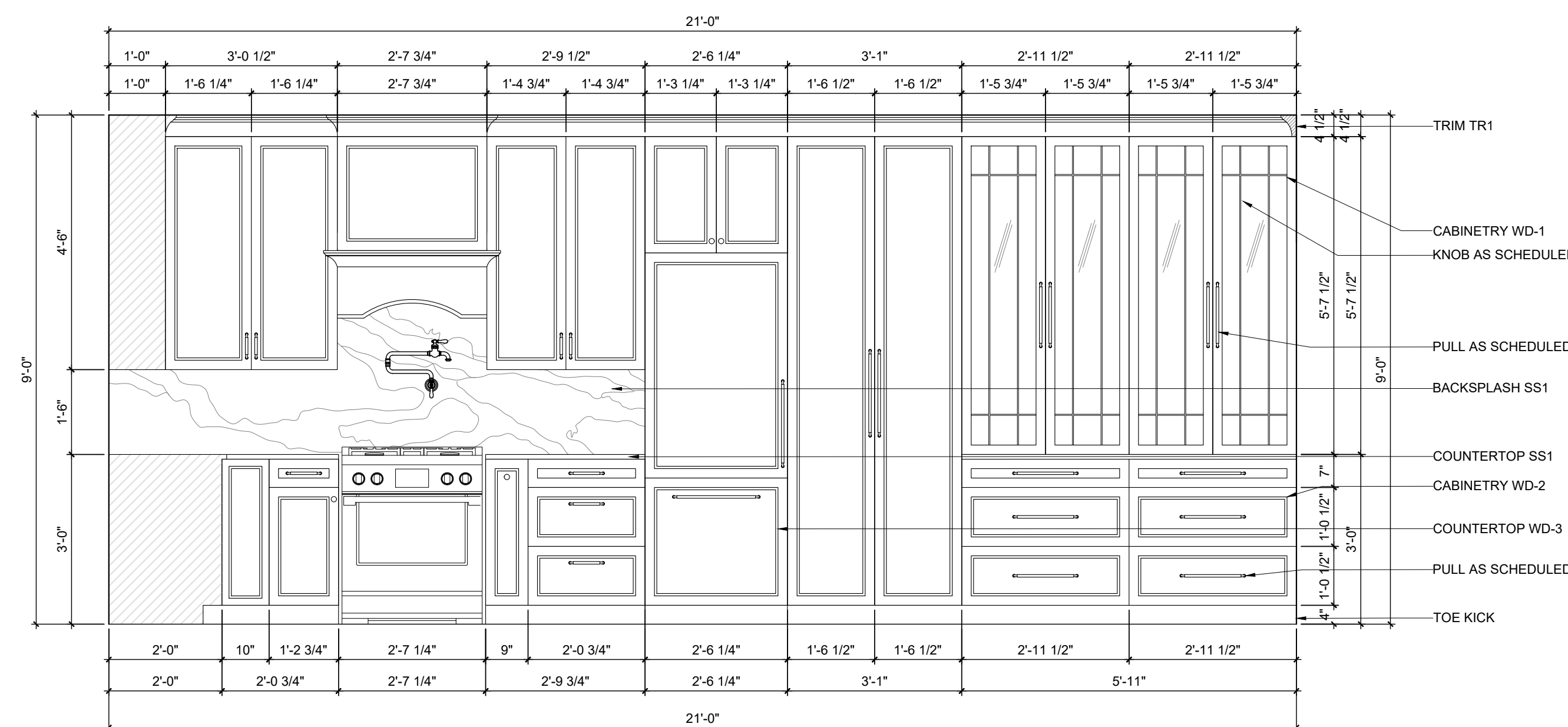
A KITCHEN STOVE ELEVATION SCALE: \frac{1}{8}" = 1' - 0"
