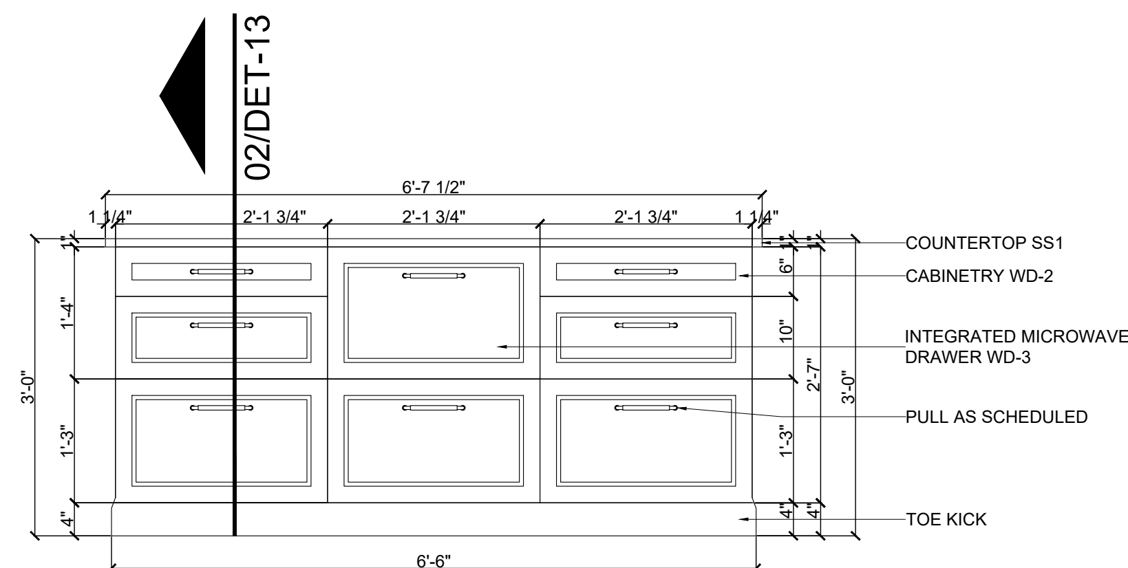
F FRONT ISLAND ELEV. SCALE: \frac{1}{8}" = 1' - 0"
