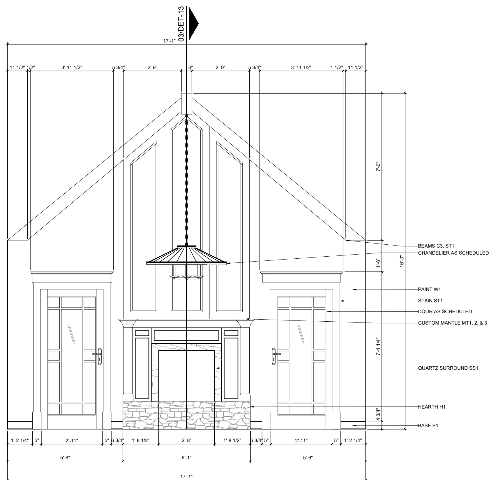
H FIREPLACE ELEVATION SCALE: \frac{1}{8}" = 1' - 0"
