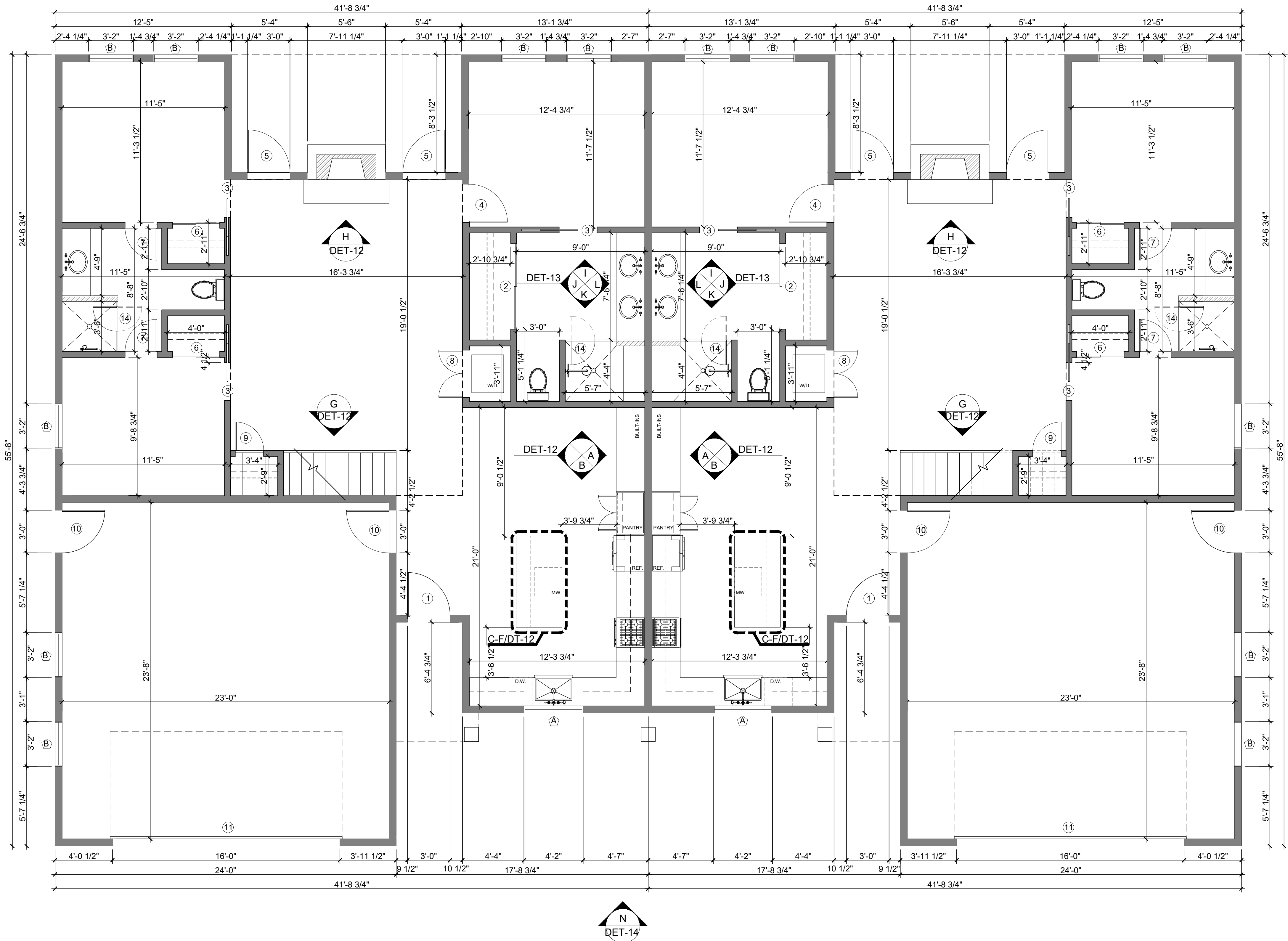
01 FIRST FLOOR PLAN SCALE: \frac{1}{4}" = 1' - 0"
