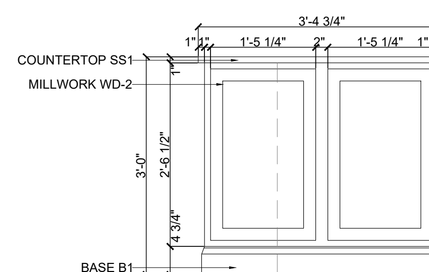
C SIDE ISLAND ELEV. SCALE: \frac{1}{8}" = 1' - 0"
