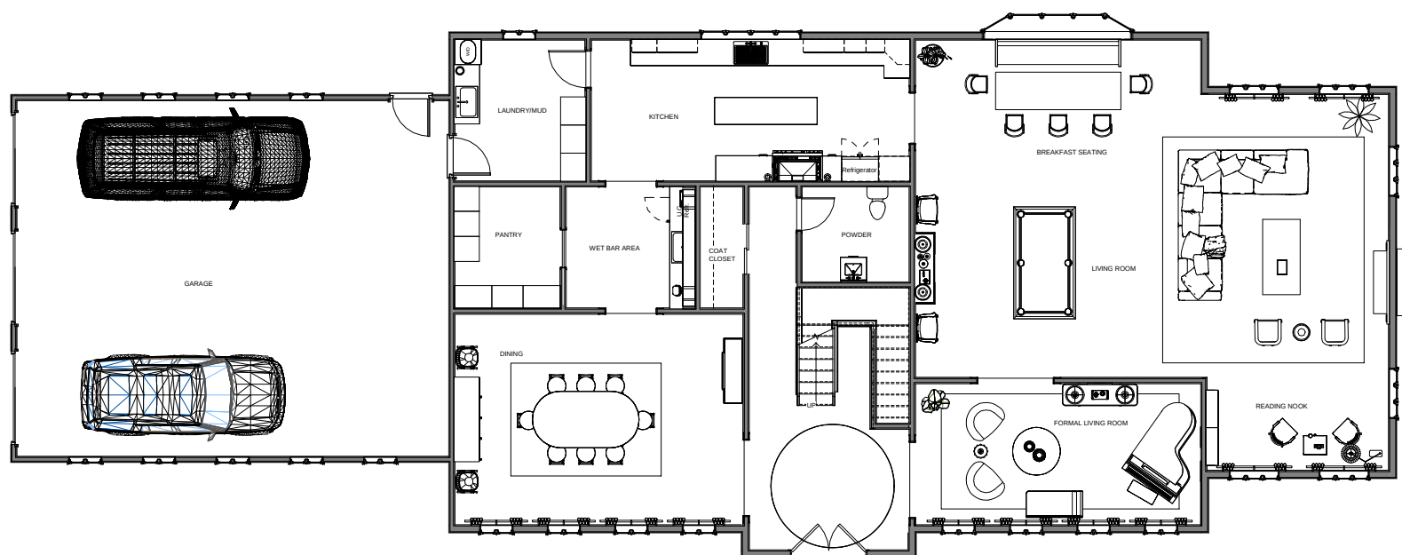
① First Floor Furniture Plan 1/4" = 1'-0"
