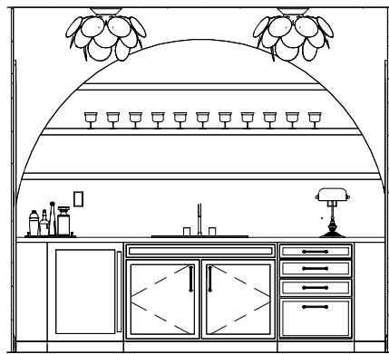
④ Wet Bar Elevation 3/4" = 1'-0"
