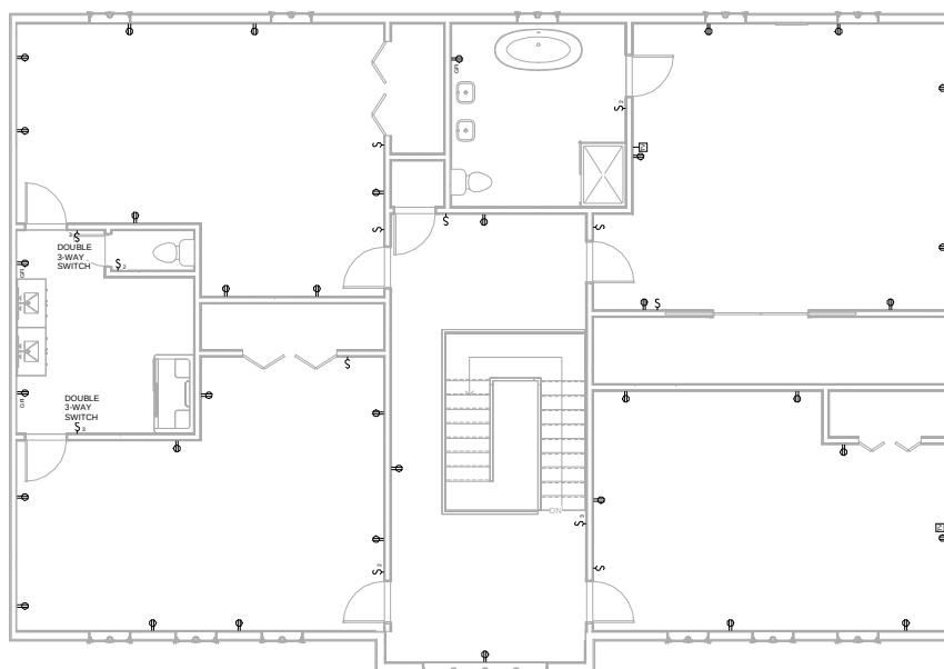
① Second Floor Electrical 1/4" = 1'-0"
