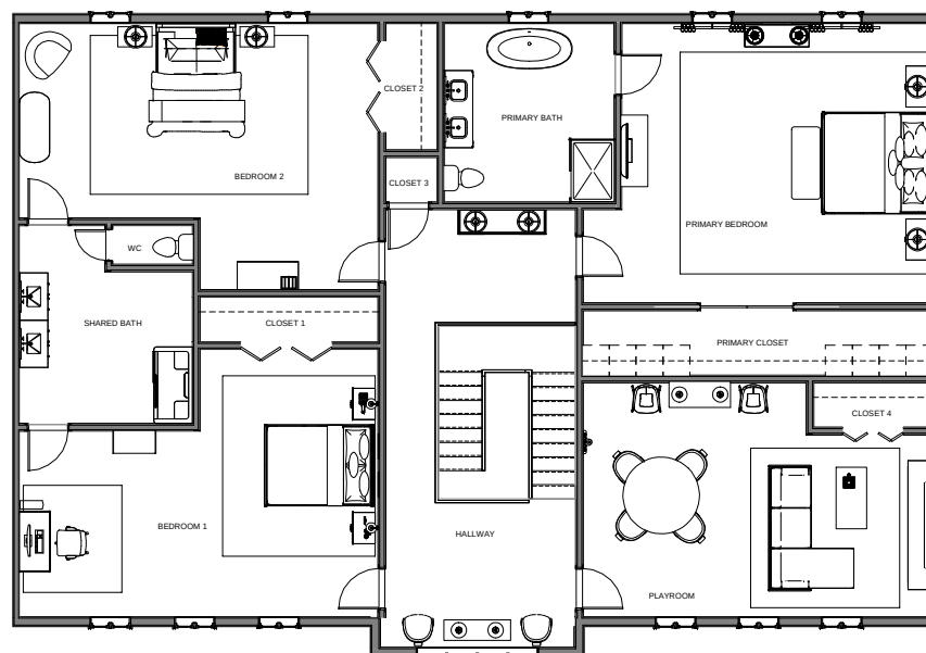
① Second Floor Furniture Plan 1/4" = 1'-0"
