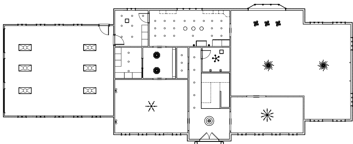
① First Floor Ceiling Plan 3/16" = 1'-0"
